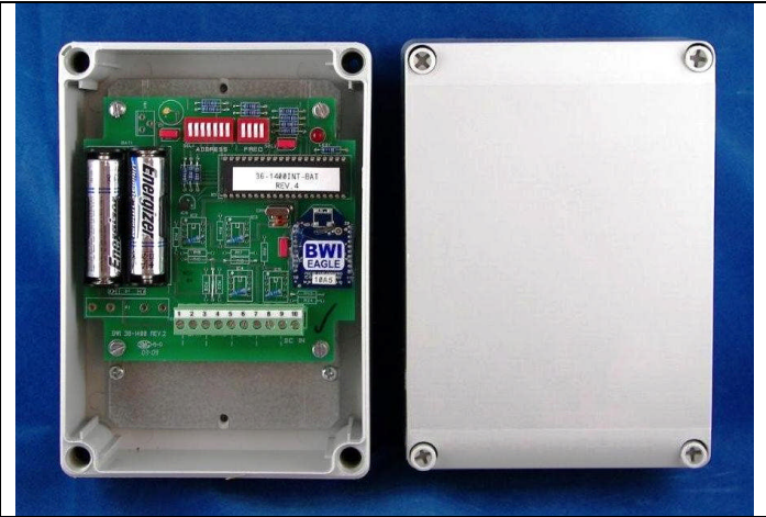
Dimensions (with mounting plate) 6 3/4" L x 4 7/8" W x 3 7/8" H
