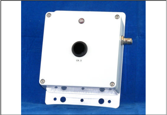
(Similar Model 36-1400-1B-BAT Shown) Dimensions (with mounting plate) 6.3" L x 4.8" W x 2.3" H
